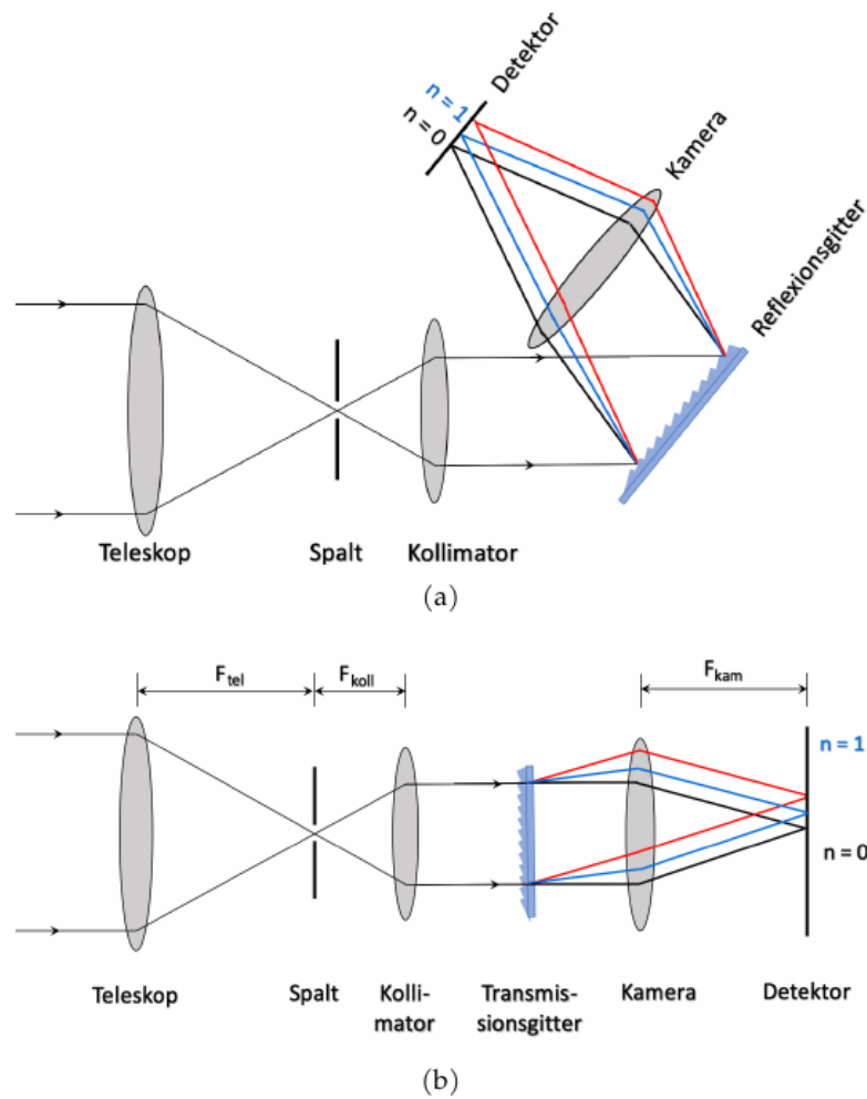
Figure 3: Schematic overview of a slit spectrograph. After entering the instrument through a slit, which here serves as the system's entrance pupil, the light is dispersed at the dispersive element ( top : reflective grating; bottom : transmissive grating). The spectrum is then focused by the camera onto the detector, where the final image is recorded. The choice of the dispersive element does not change the basic set-up. Credit: V. Pfeiffer (2020).
