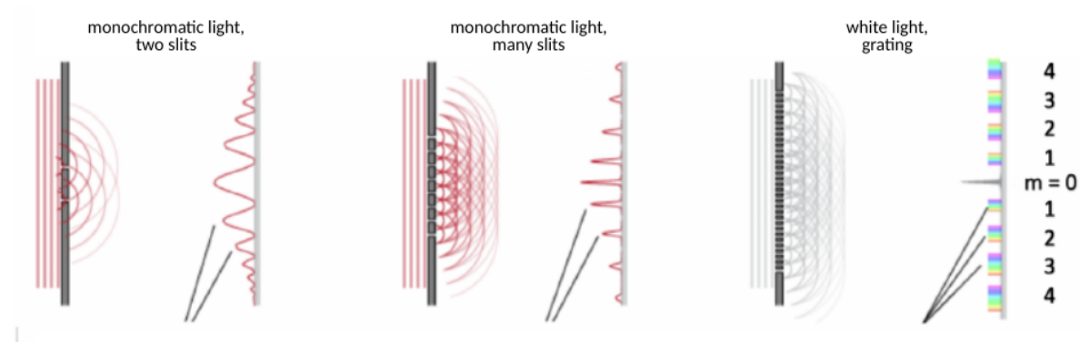
Figure 5: Different diffraction patterns. Left : Monochromatic light through two slits. Middle : Monochromatic light through many slits. Right : Polychromatic light through a grating. With increasing number of illuminated slits the interference peaks become narrower, therefore the resolving power increases. While there is no dispersion at the 0th order, the angular dispersion increases with spectral order. Credit: V. Pfeiffer (2020).
